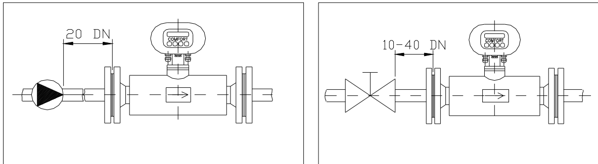
Straight piping sections to stabilise the fluid flow after a "disturbance" in the piping
