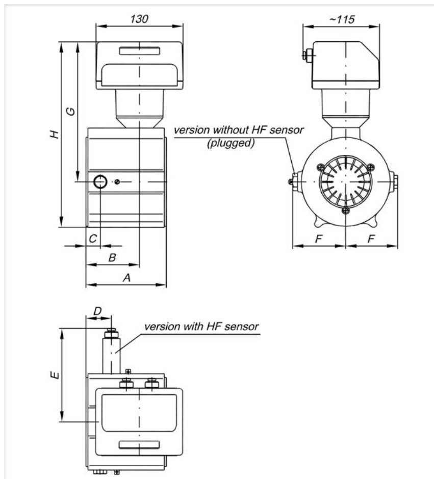
Fig.12. Basic dimensions of the CPT-01 Quantometers
